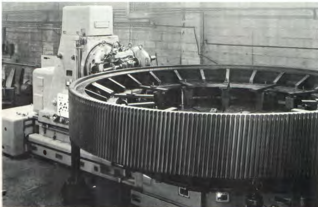
200" Gear Hobber produces helical and spur gears up to 28" face
