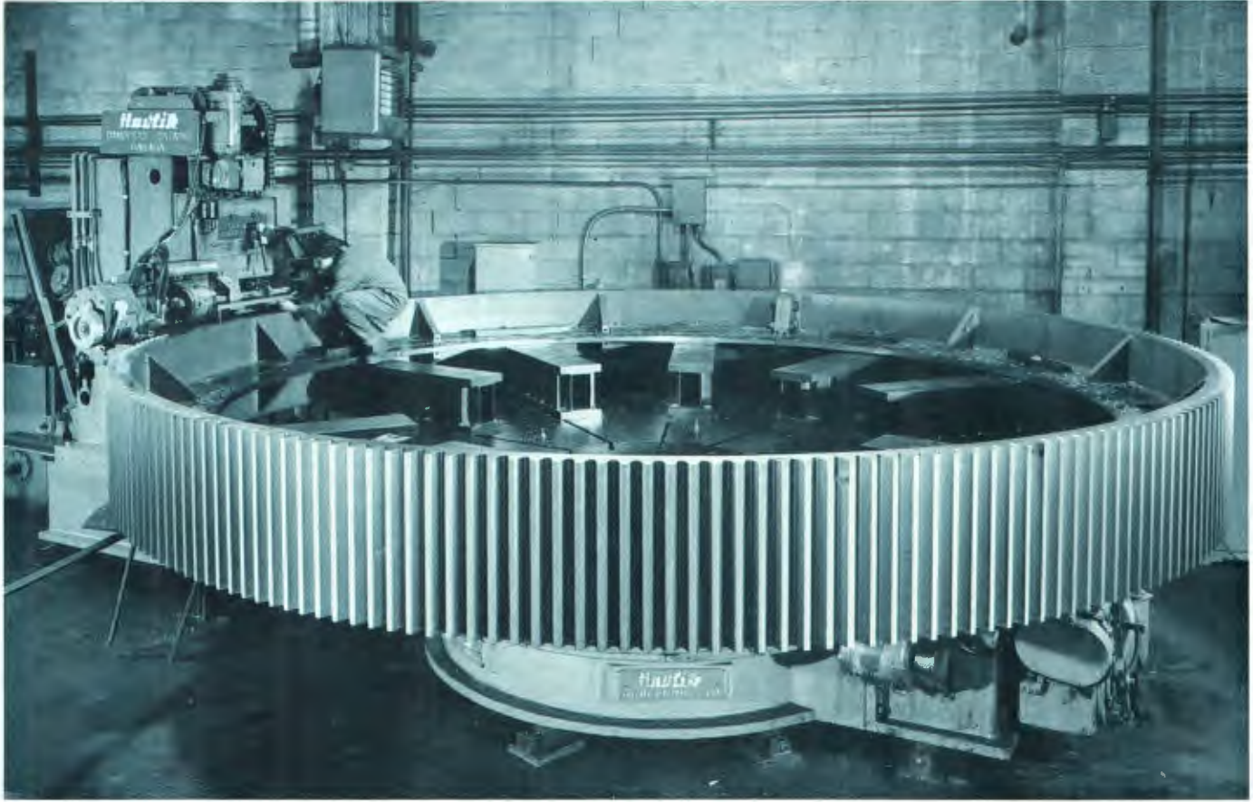
This picture portrays a gear manufactured by True Forge Limited and was approximately 220" in diameter with a 24" face.
